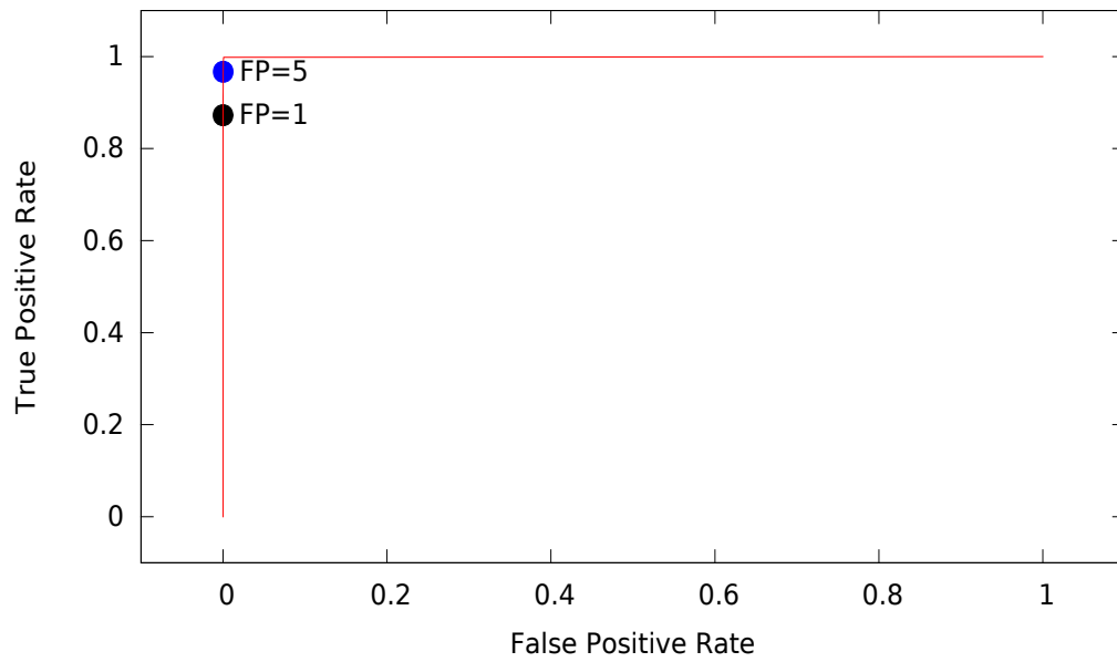
ROC graph for H3
