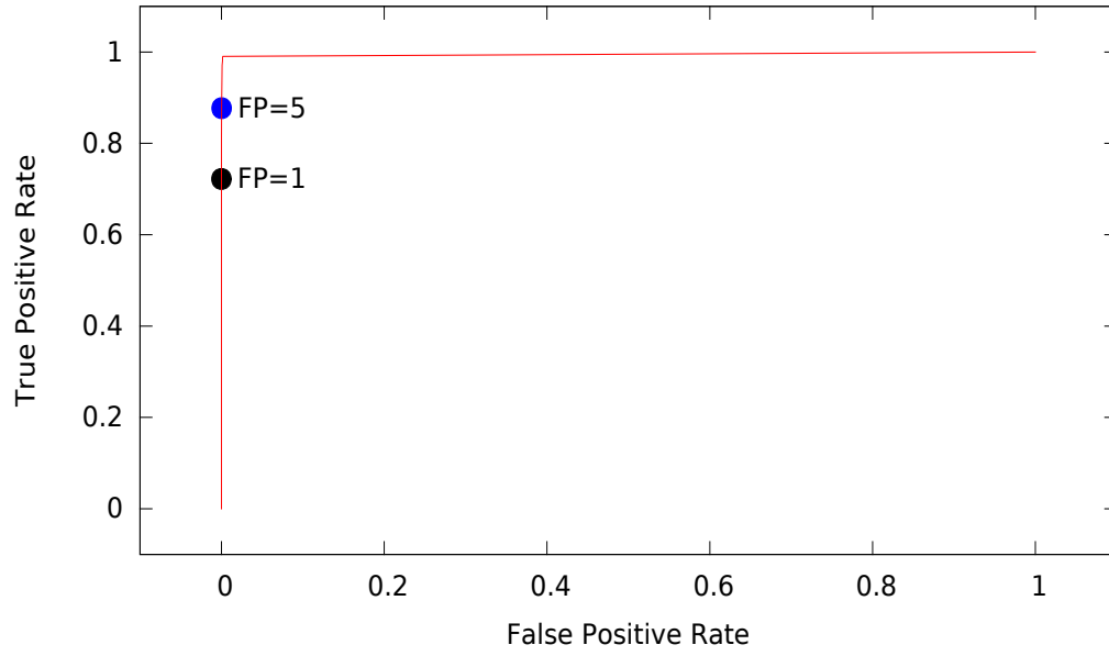
ROC graph for H2
