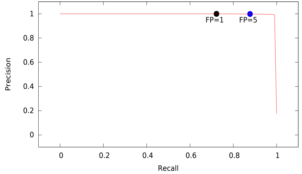
Precision-Recall graph for H2
