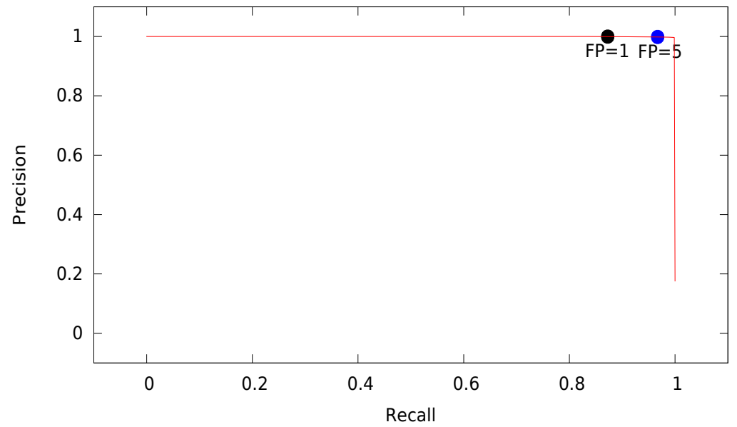
Precision-Recall graph for H3
